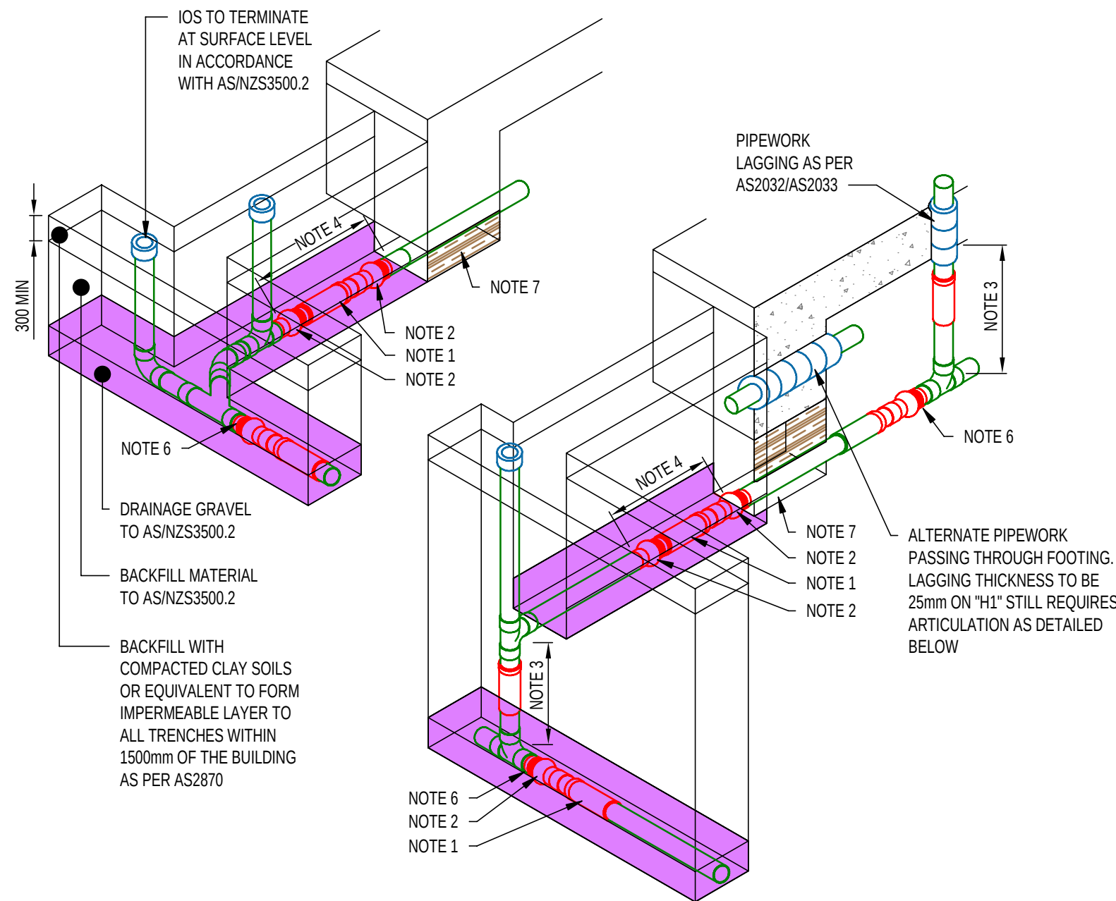
1 IN GROUND DRAINAGE (STORMWATER & SANITARY) N.T.S.
